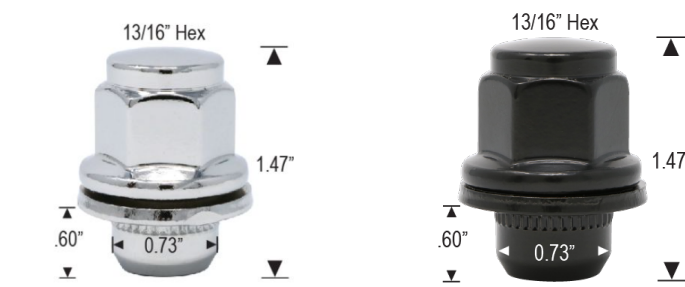
MEDIUM MAG W/ATTACHED WASHER
