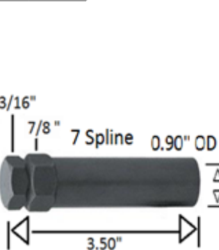
7PT SPLINE KEY
