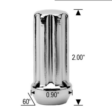
XL SPLINE 7PT
