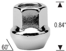
OPEN END ACORN
