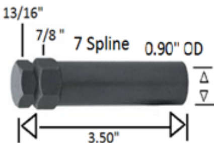
7PT SPLINE KEY
