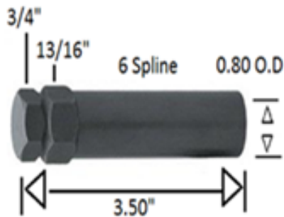
6PT SPLINE KEY
